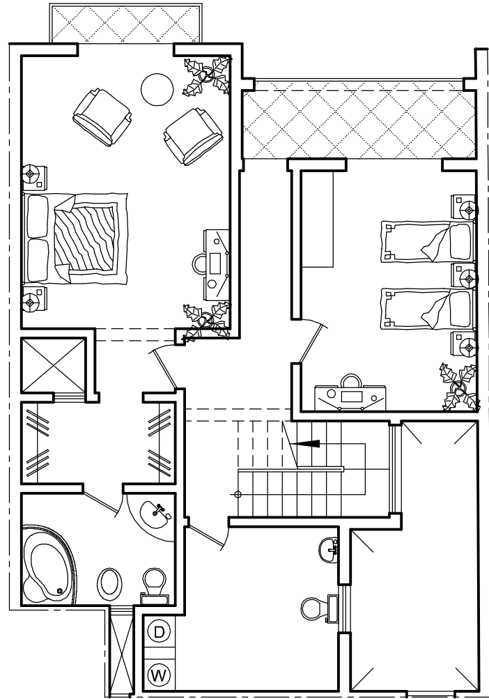
PENTHOUSE BOTTOM FLOOR PLAN 1:100
